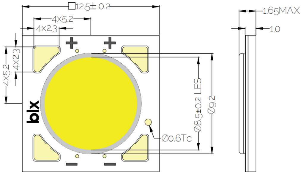
Figure 15: Drawing for V8 LED Array
