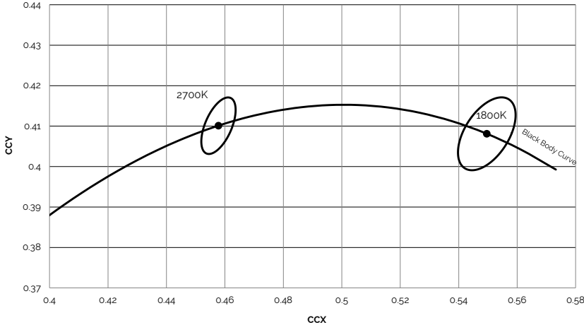
Figure 20: Graph of Warm White Test Bins in xy Color Space, T_c = 25^\circ\text{C}
