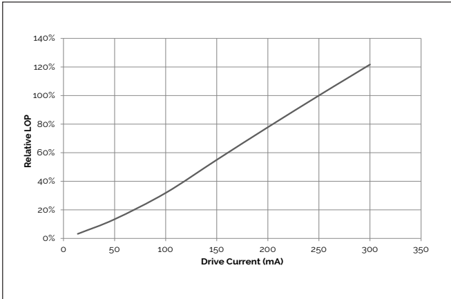
Figure 9: 4W Relative LOP vs. Drive Current, T_c=25^\circ\text{C}
