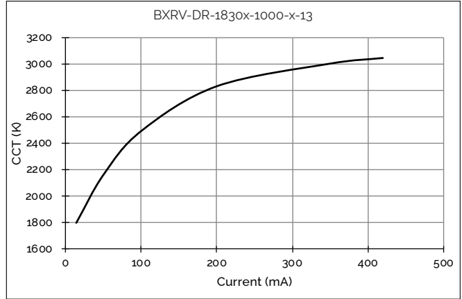
Figure 8: 12W CCT vs. Forward Current, T_c=25^\circ\text{C}
