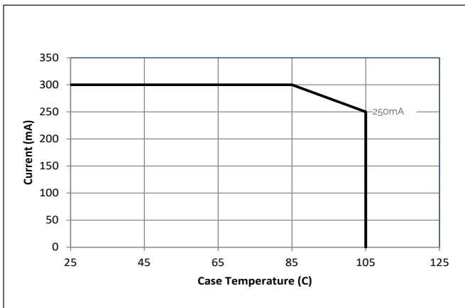
Figure 14: Derating Curve 4W
