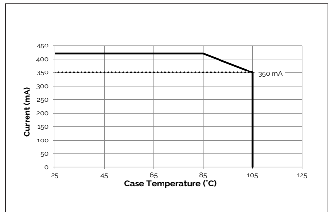
Figure 15: Derating Curve 6W, 12W
