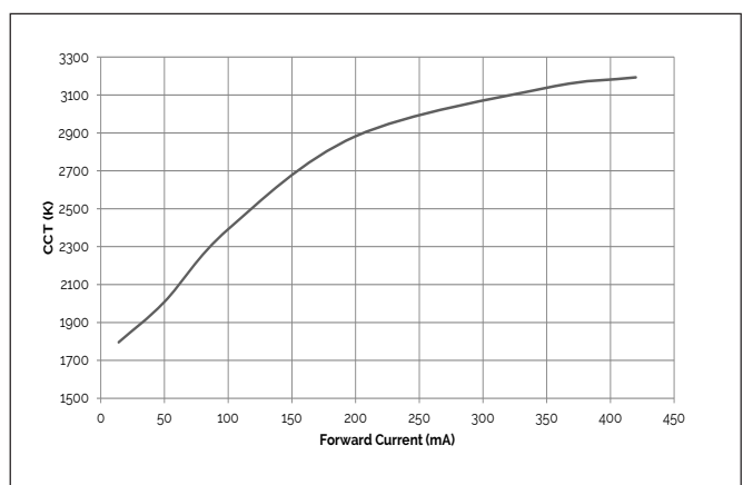
Figure 6: 6W CCT vs. Forward Current, T_c = 25^\circ\text{C}
