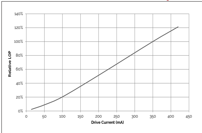
Figure 11: 12W Relative LOP vs. Drive Current, T_c=25^\circ\text{C}
