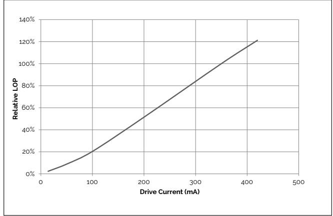
Figure 10: 6W Relative LOP vs. Drive Current, T_c=25^\circ\text{C}
