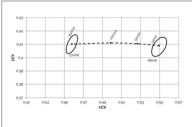
Figure 12: Color shift vs. Forward Current 2700K - 1800K
