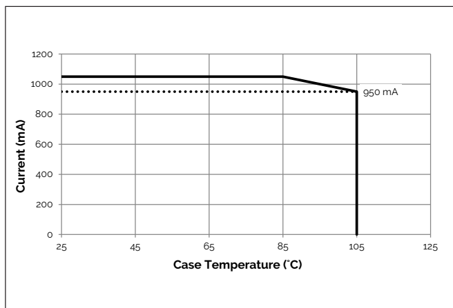
Figure 8: Derating Curve
