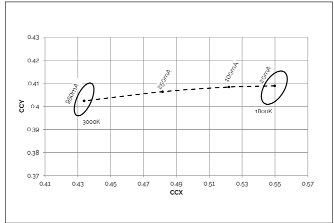
Figure 4: Color Shift vs. Forward Current 3000K-1800K
