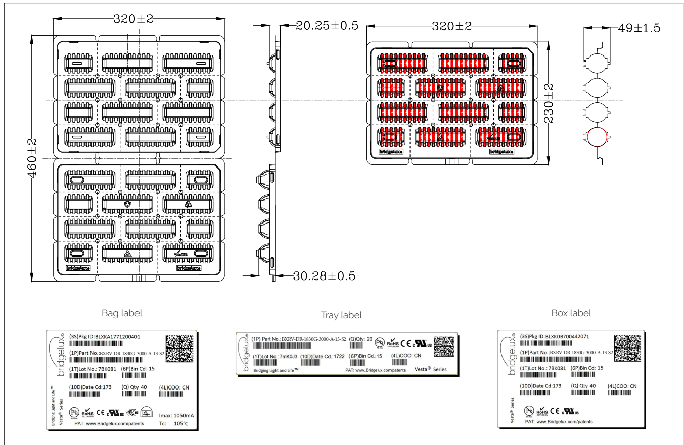
Figure 14: Packaging Specifications
