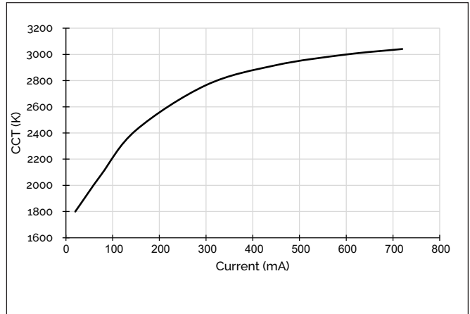
Figure 2: CCT vs. Forward Current 3000K-1800K
