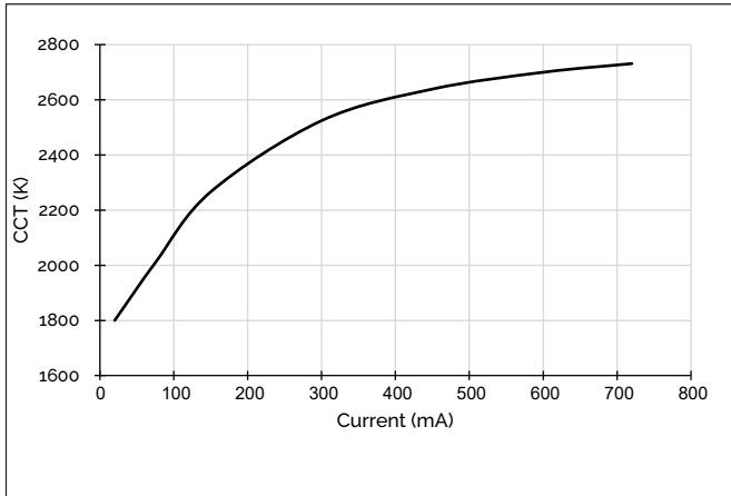
Figure 1: CCT vs. Forward Current 2700K - 1800K
