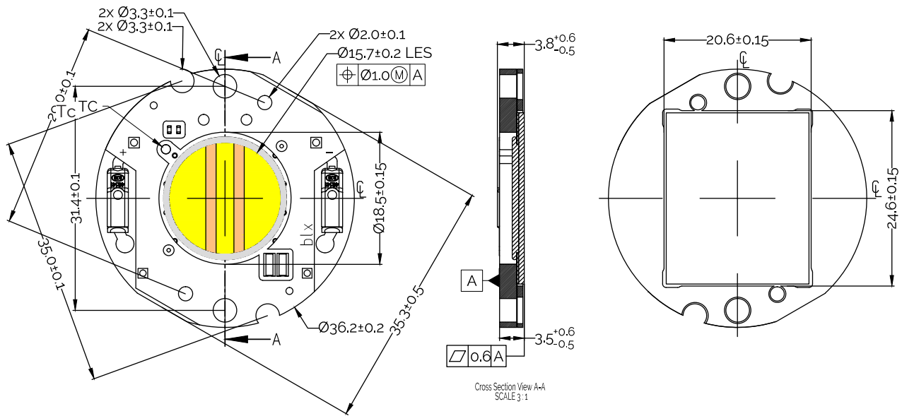
Figure 12: Mechanical Drawing Specification
