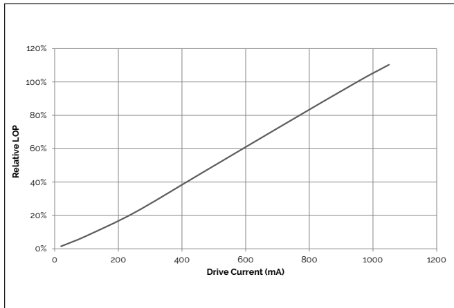
Figure 6: Relative LOP vs. Drive Current, T_c=25^\circ\text{C}
