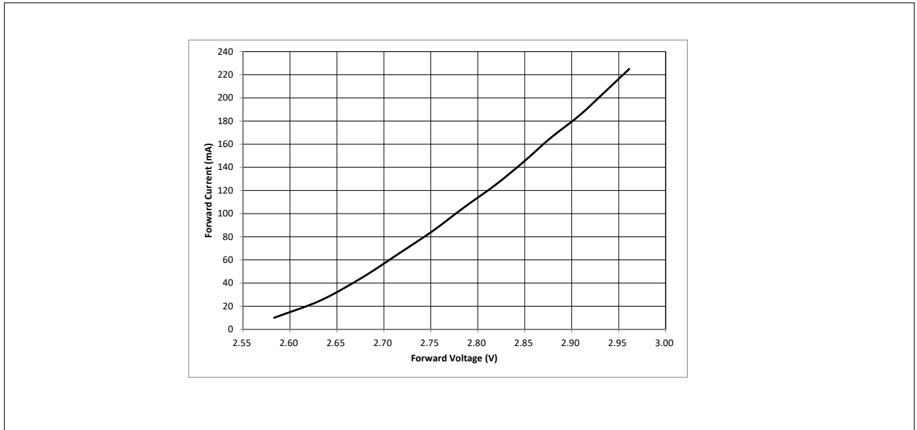
Figure 2: Test Current vs. Voltage ( T_{sp}=25^{\circ}\text{C} )
