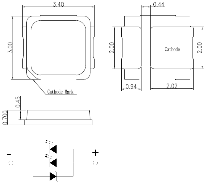
Figure 10: Drawing for SMD 3030
