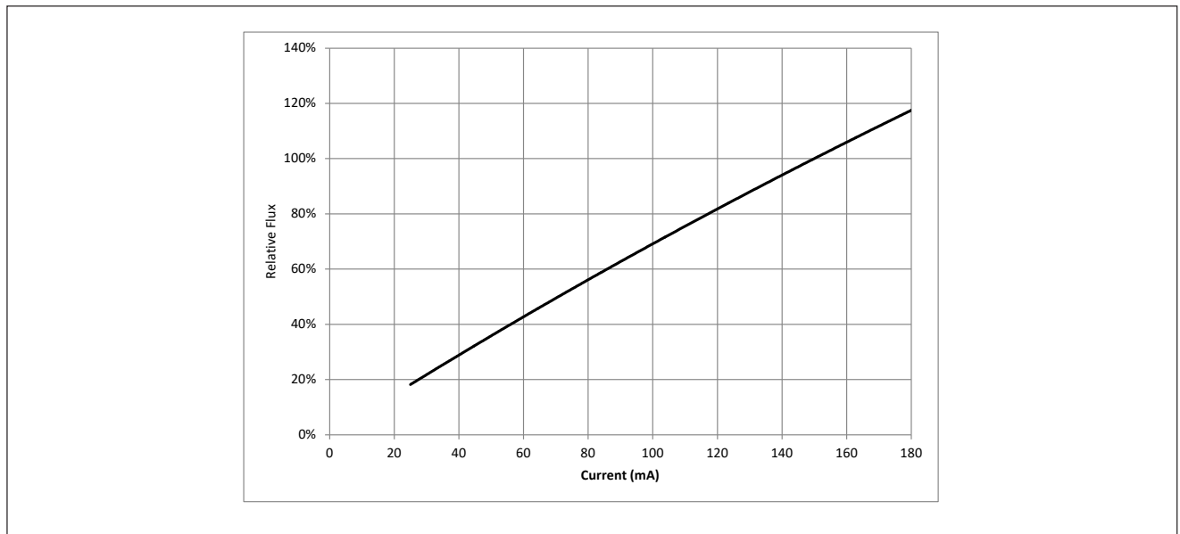
Figure 3: Typical Relative Luminous Flux vs. Drive Current ( T_{sp}=25^{\circ}\text{C} )
