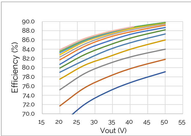
Figure 10: Efficiency @ 347VAC
