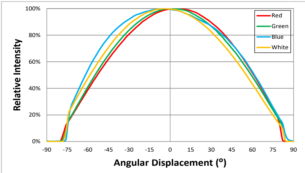
Figure 7: Typical Spatial Radiation Pattern at 120mA, T_{sp}=25^{\circ}\text{C}
