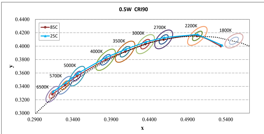
Figure 5: Chromaticity Coordinate Group(Color Targeted at T_{sp} = 25^{\circ}\text{C} & 85^{\circ}\text{C} )
