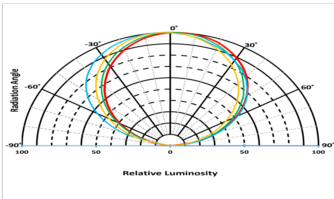
Figure 8: Typical Polar Radiation Pattern at 120mA, T_{sp}=25^{\circ}\text{C}
