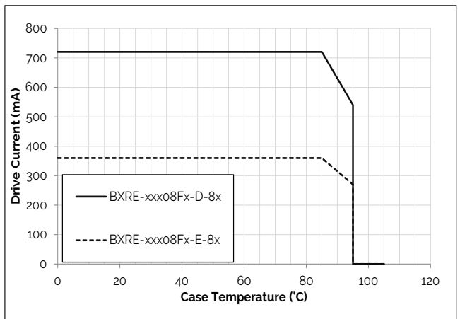
Figure 12: Derating Curve
