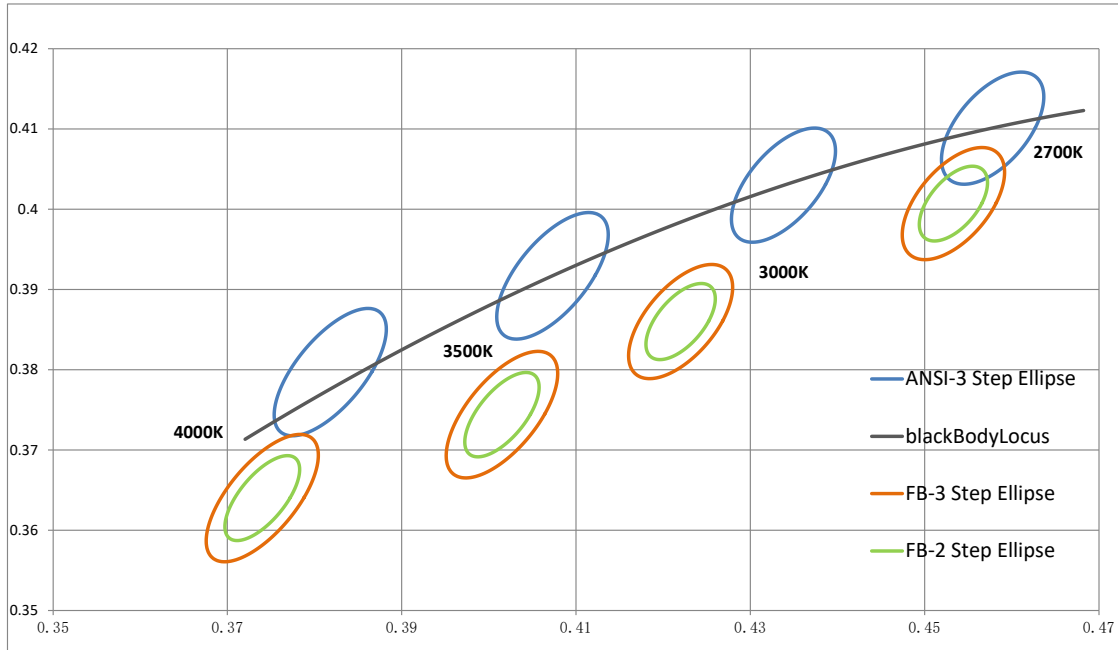
Figure 11: Warm White Test Bins in xy Color Space
