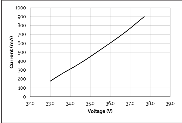
Figure 3: V13C Drive Current vs. Voltage
