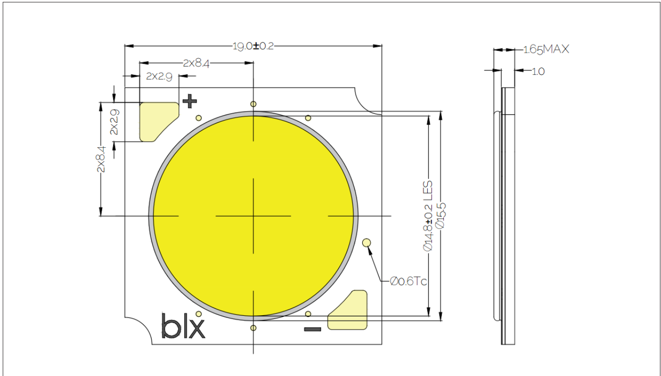
Figure 10: Drawing for V13 LED Array
