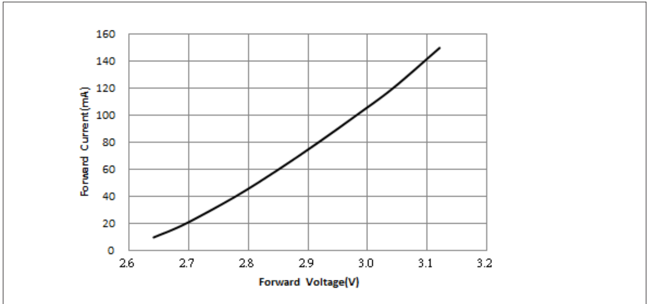
Figure 2: Forward Current vs. Forward Voltage ( T_{sp}=25^{\circ}\text{C} )
