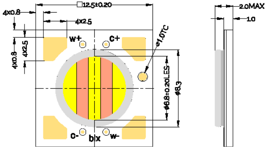
Figure 20: Mechanical Drawing Specifications : BXRV-TR-1840X-06A0-B-2X
