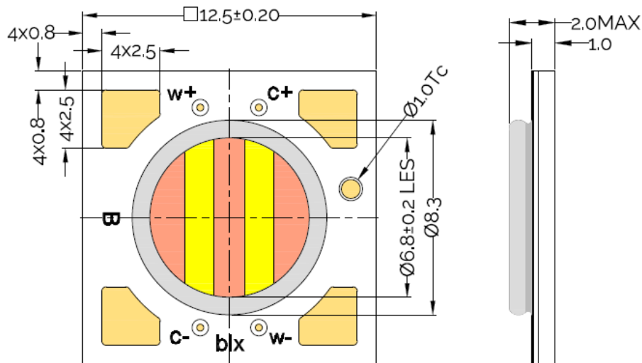
Figure 20: Mechanical Drawing Specifications : BXRV-TR-1840X-06A0-B-2X
