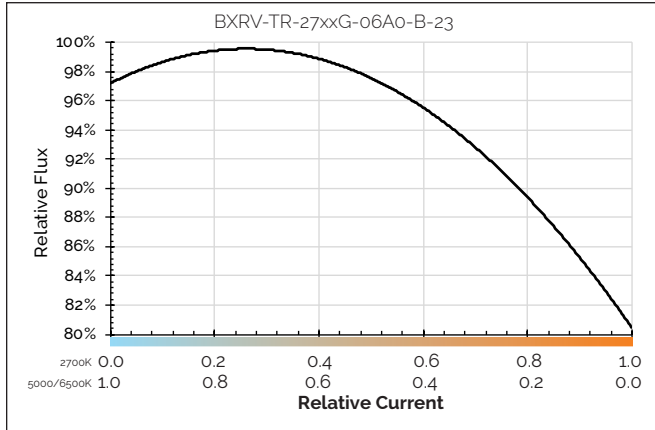
Figure 9: Relative Flux vs. Relative Current
