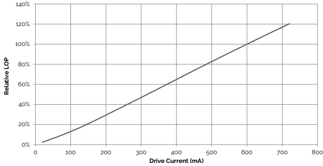
Figure 6: Relative LOP vs. Drive Current, T_c=25^\circ\text{C}
