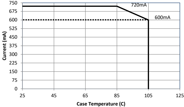
Figure 8: Derating Curve
