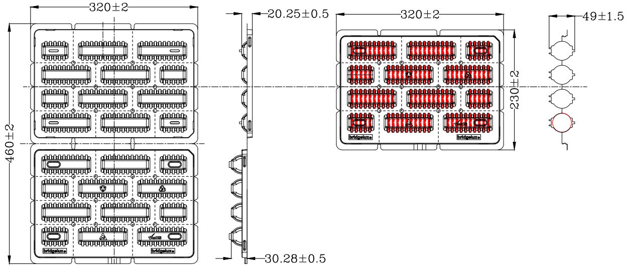
Figure 14: Packaging Specifications
