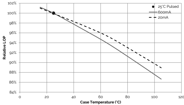
Figure 7: Relative Flux vs. Case Temperature
