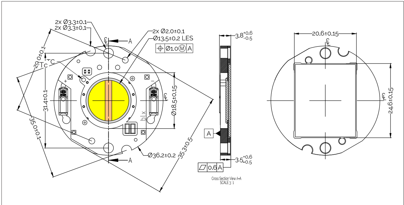
Figure 12: Mechanical Drawing Specification
