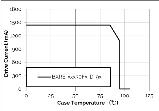
Figure 8: Derating Curve
