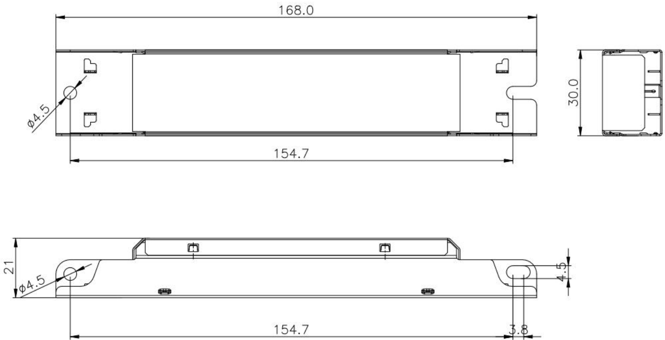
Figure 6: Mechanical Drawing
