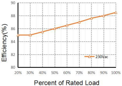
Figure 3: Efficiency vs. Load
