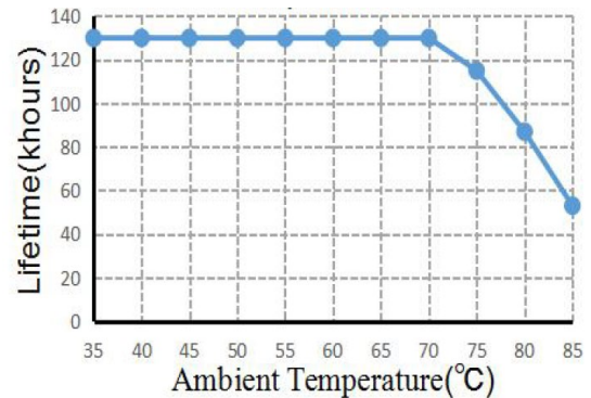
Figure 4: Expected Life Time
