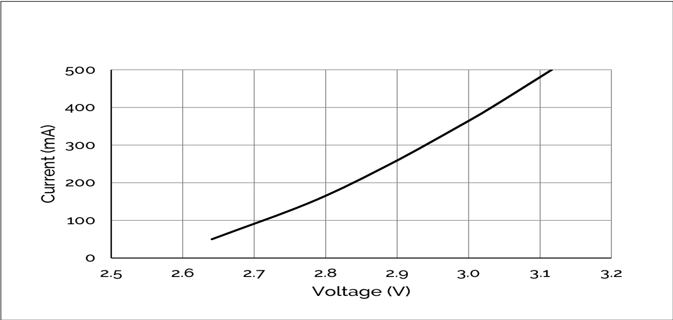
Figure 2: Drive Current vs. Voltage ( T_{sp}=85^{\circ}C )
