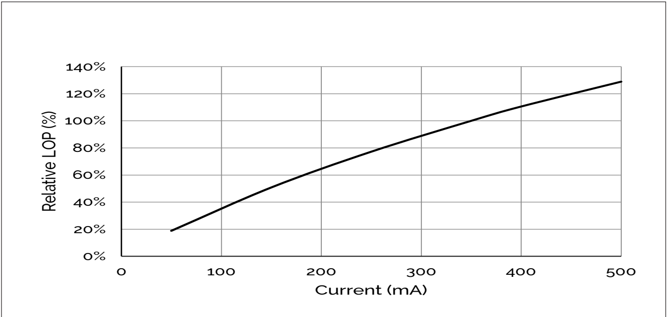
Figure 3: Typical Relative Luminous Flux vs. Drive Current ( T_{sp}=85^{\circ}C )
