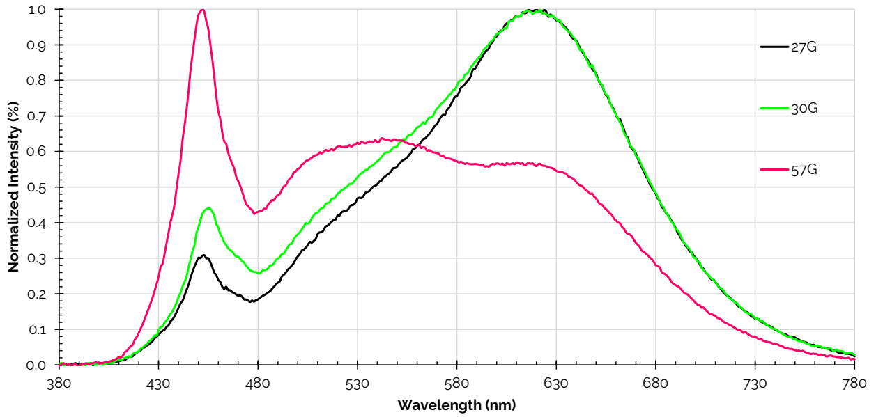
Figure 10: Typical Color Spectrum at 350mA, Tsp=85°C
