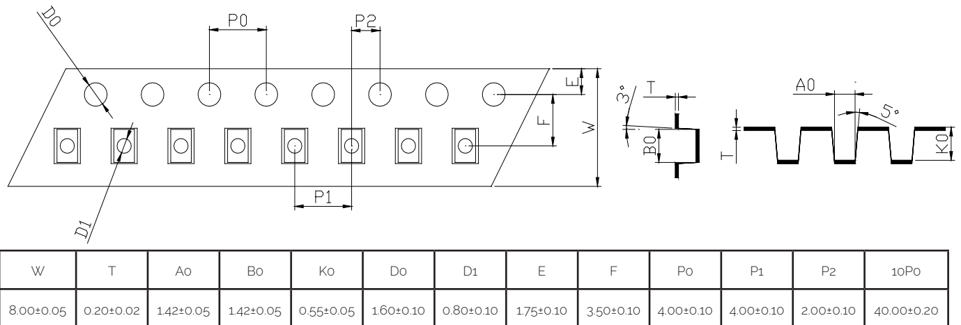
Figure 14: Tape Drawings
