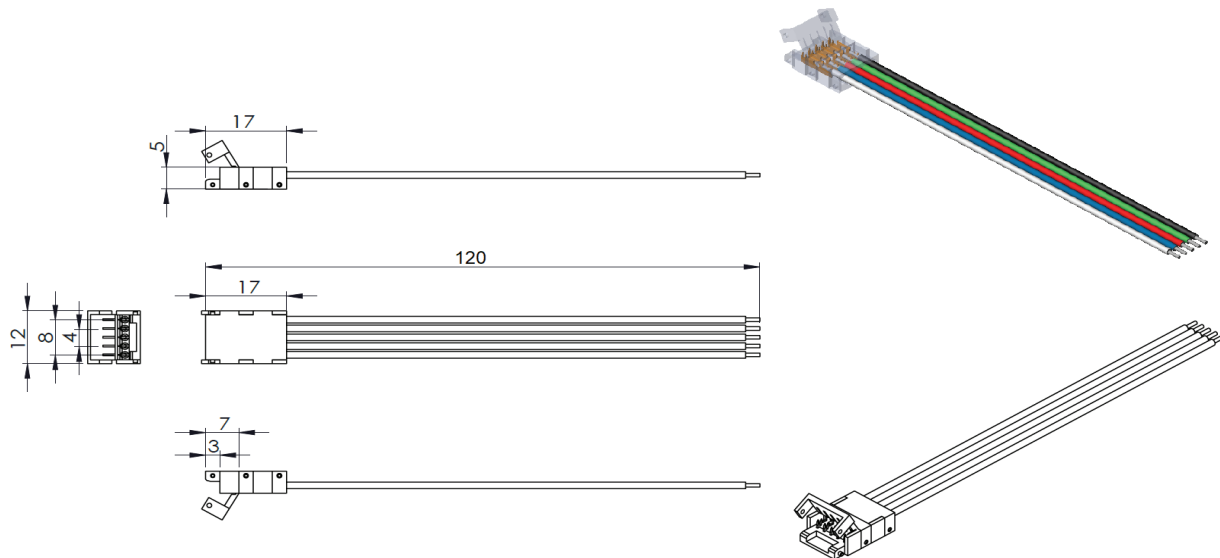
Figure 14: Mechanical Drawing for BXCN-RGBW-L120-SH
