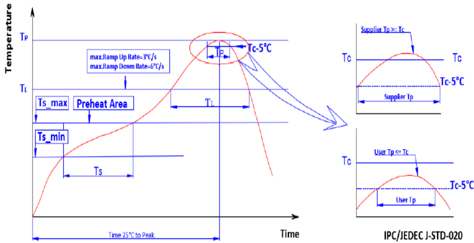
Figure 24 : Reflow Profile
