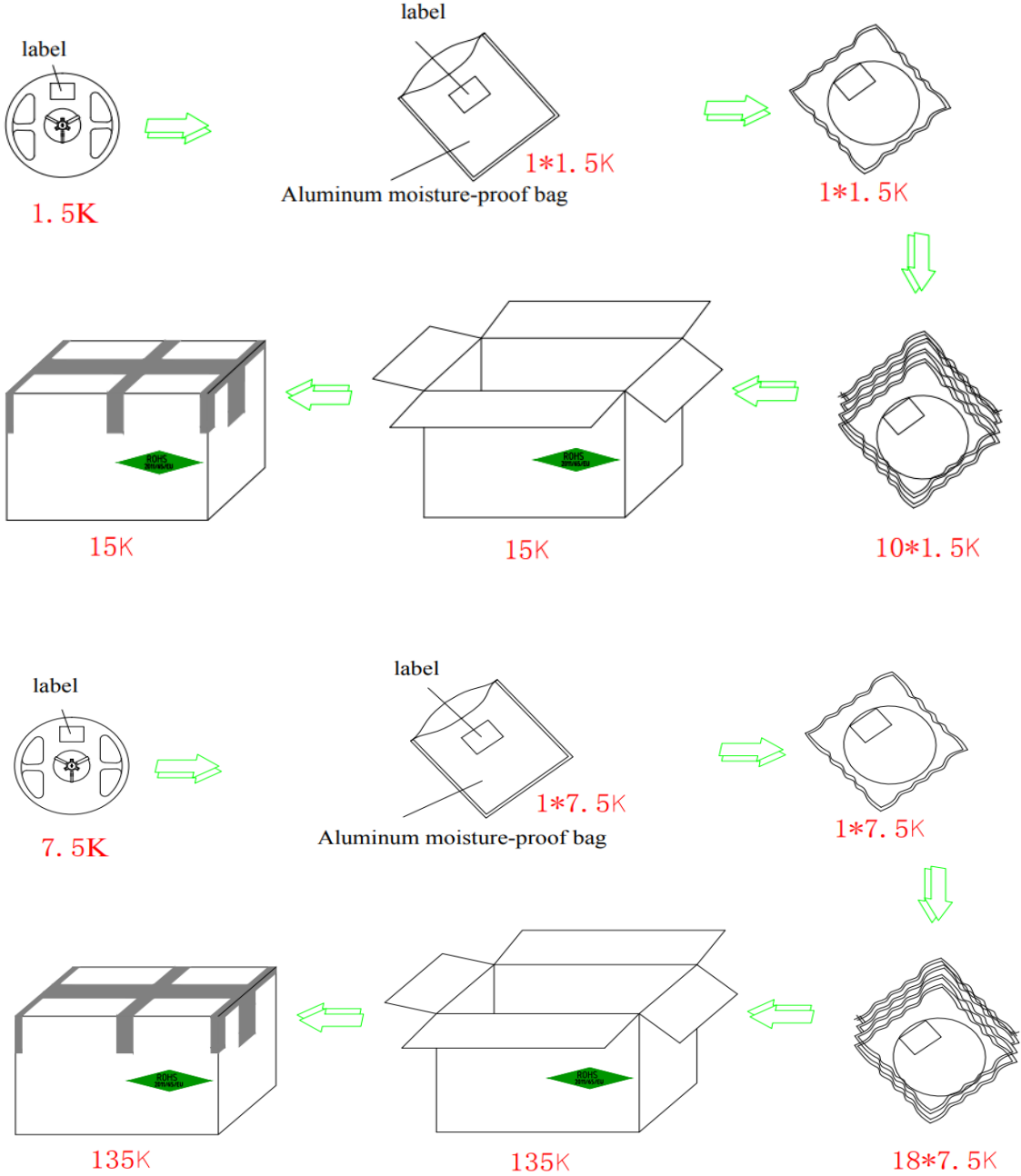
Figure 27: Emitter Reel Packaging Drawings
