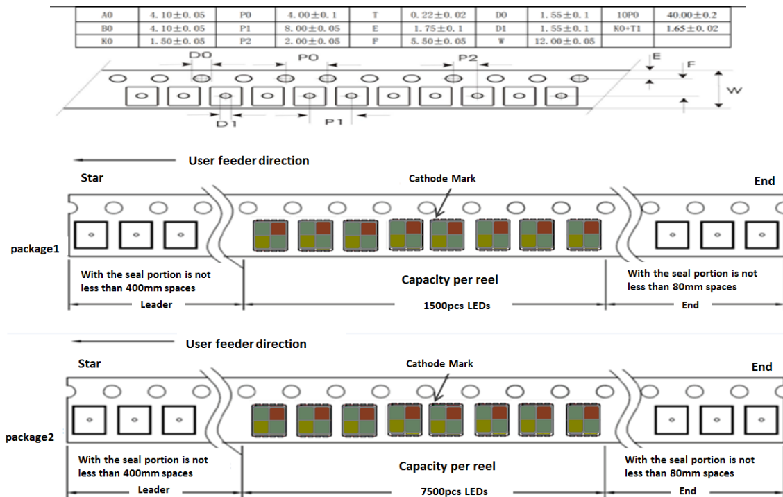
Figure 26: Emitter Tape Drawings
