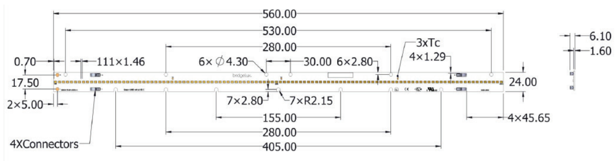
Figure 19: Drawing Overview for 560mm
