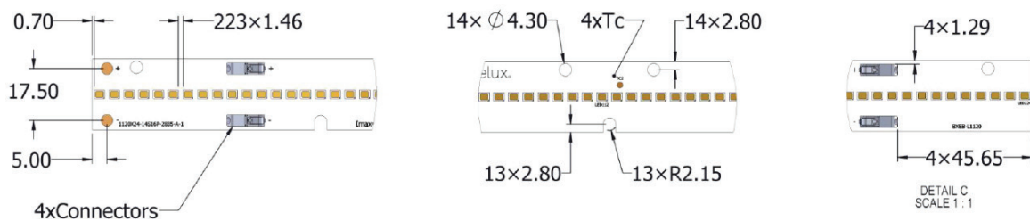
Figure 20: Drawing Overview for 1120mm
