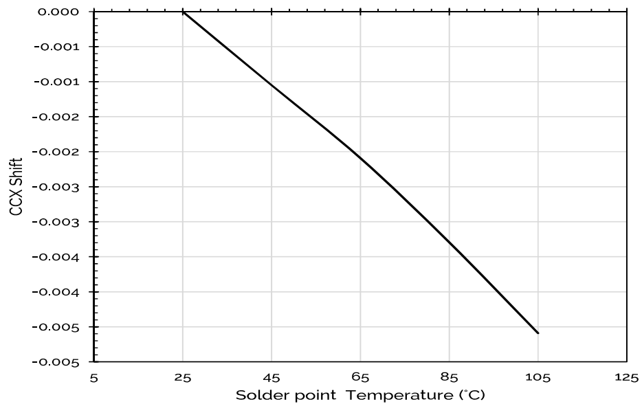
Figure 5: Typical ccx Shift vs. Solder Point Temperature
