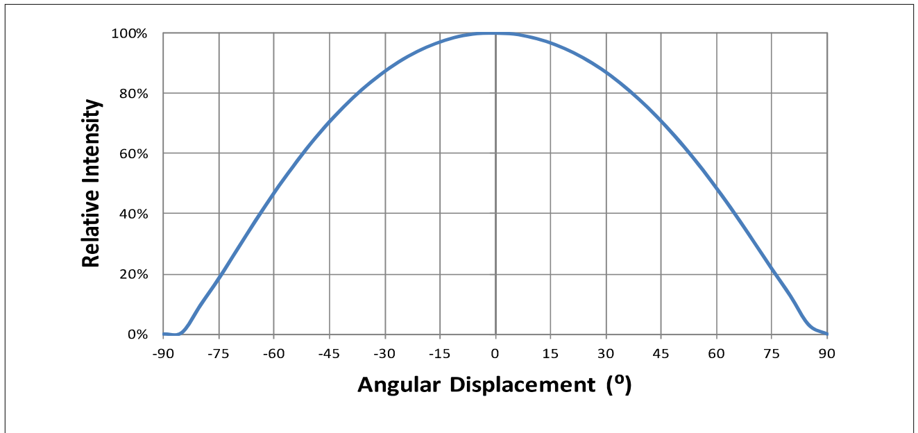
Figure 8: Typical Spatial Radiation Pattern at 65mA, T_{sp}=25^{\circ}\text{C}
