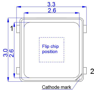
Figure 11: Drawing for SMD 3030
