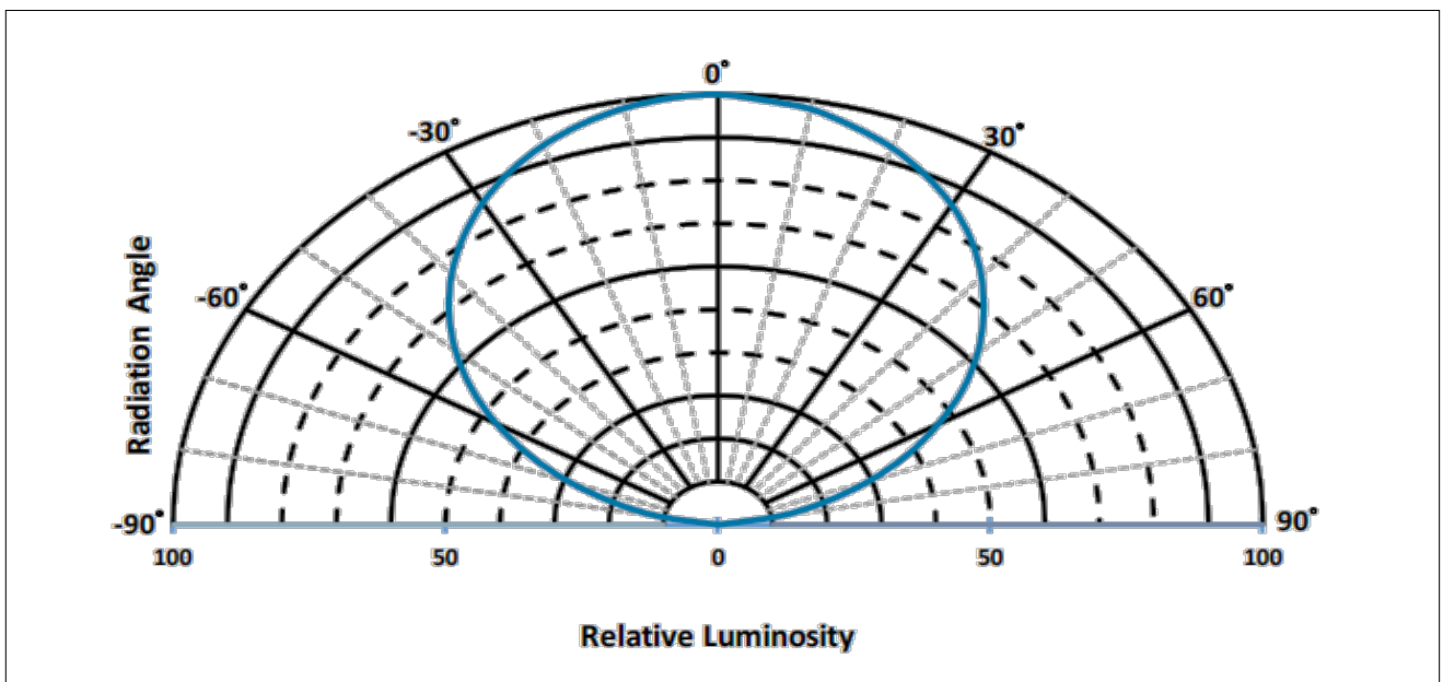
Figure 9: Typical Polar Radiation Pattern at 65mA, T_{sp} = 25^{\circ}\text{C}
