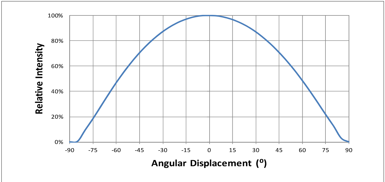
Figure 8: Typical Spatial Radiation Pattern at 65mA, T_{sp} = 25^{\circ}\text{C}
