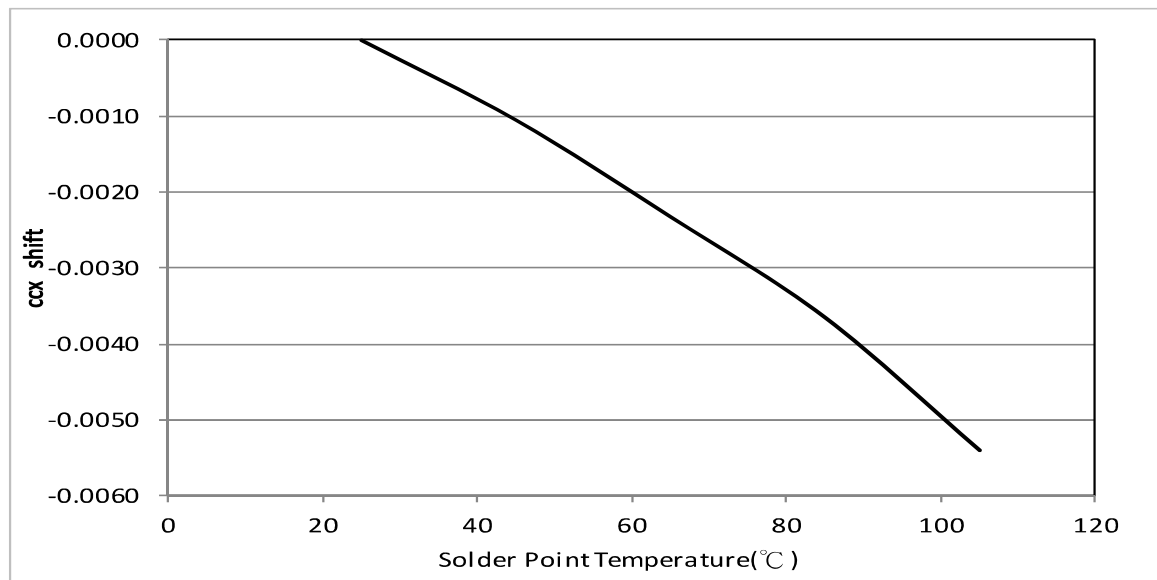
Figure 5: Typical ccx Shift vs. Solder Point Temperature
