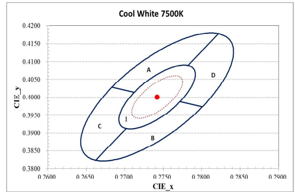
Figure 1: C.I.E. 1931 Chromaticity Diagram (5 Color Bin Structure, Hot-color Targeted at T_{sp} = 85^{\circ}\text{C} )
