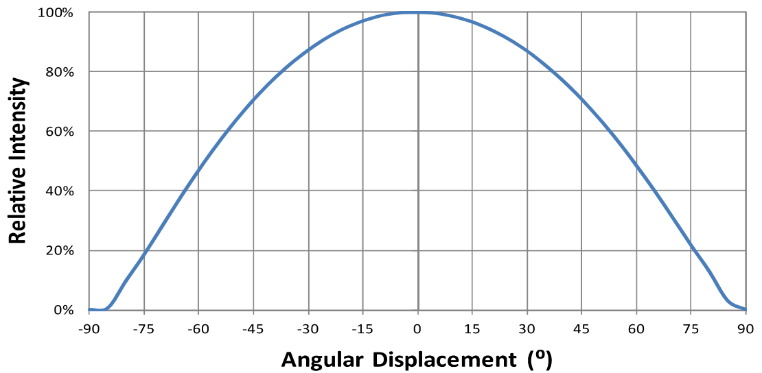
Figure 8: Typical Spatial Radiation Pattern at 65mA, T_{sp} = 25^{\circ}\text{C}
