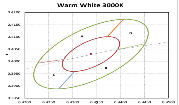
Figure 1: C.I.E. 1931 Chromaticity Diagram (5 Color Bin Structure, Hot-color Targeted at T_{sp}=85^{\circ}\text{C} )
