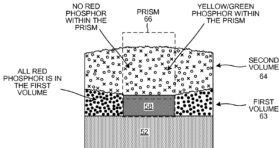
CROSS-SECTIONAL VIEW
