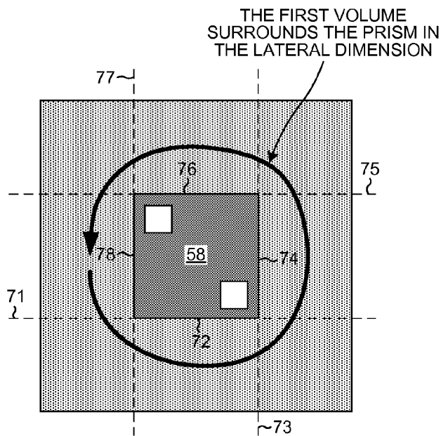
TOP-DOWN VIEW
