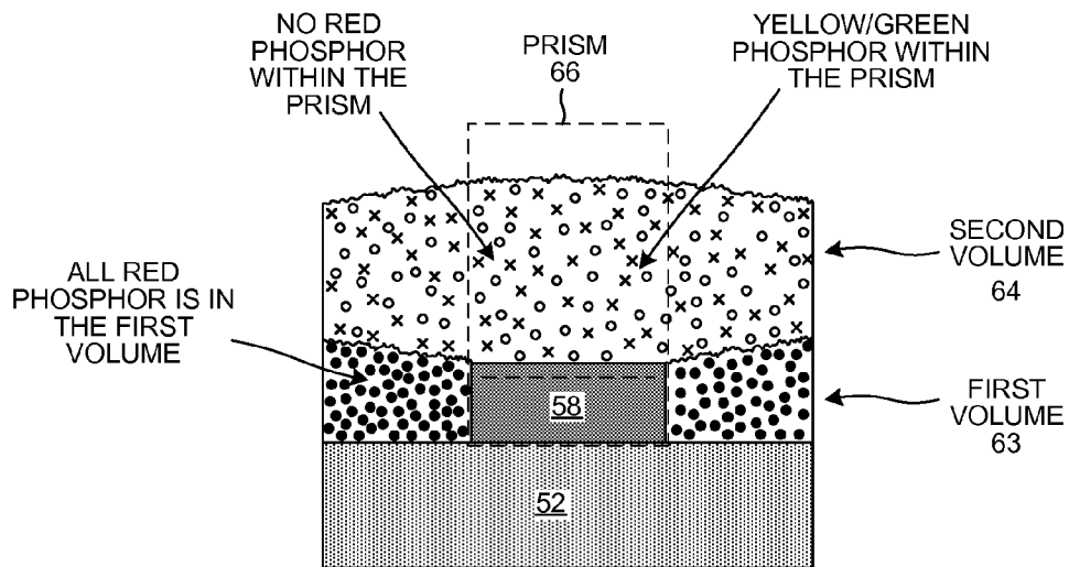
CROSS-SECTIONAL VIEW
