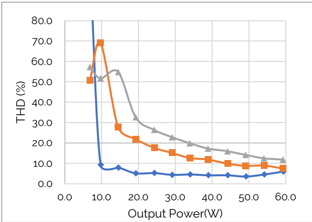
Figure 5: THD vs Output Power
