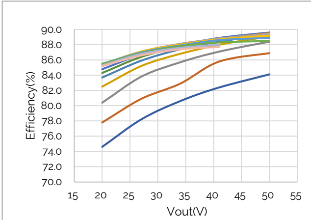
Figure 8: Efficiency @ 120VAC
