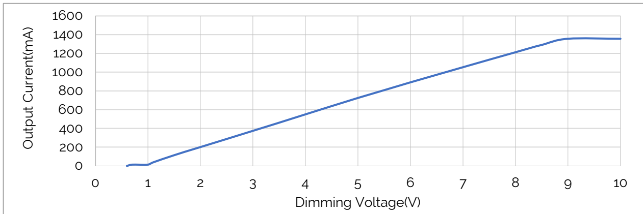
Figure 1: 0 - 10V Dimming Curve
