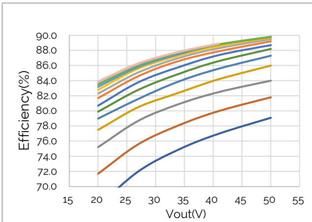
Figure 10: Efficiency @ 347VAC
