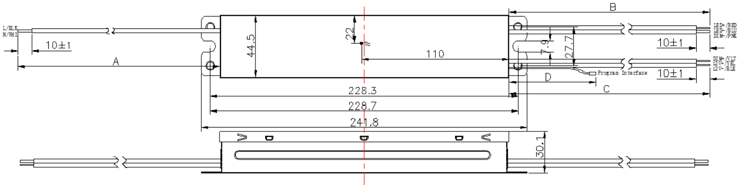
Figure 11: Mechanical Drawing
