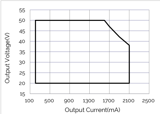
Figure 3: Operating Window
