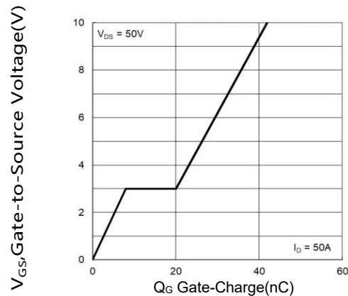
Figure6. Typical Gate Charge versus V GS
