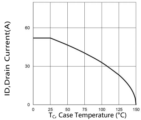
Figure10. Maximum Continuous Drain Current versus Case Temperature
