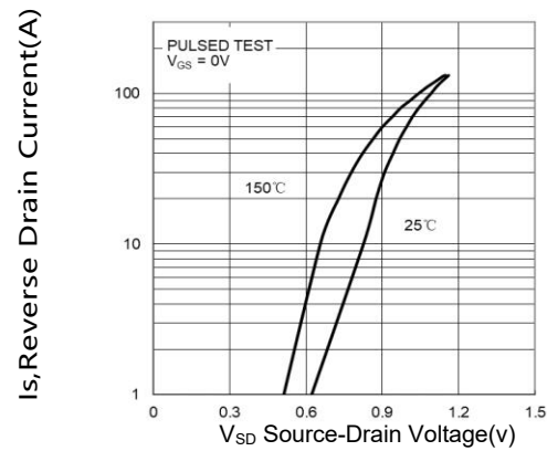
Figure4. Diode forward voltage versus Current
