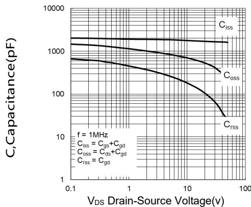
Figure5. Typical Capacitance versus V DS
