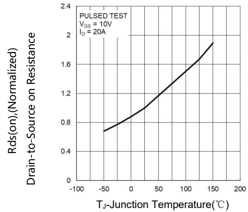
Figure8. On-Resistance Variation with Temperature
