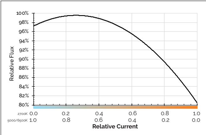
Figure 7: Relative Flux vs. Relative Current
