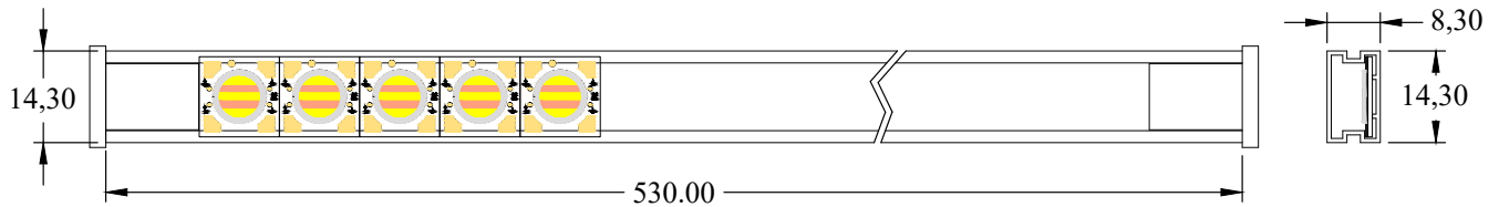
Figure 17: Vesta Series Tunable White 6mm Packaging and Labeling
