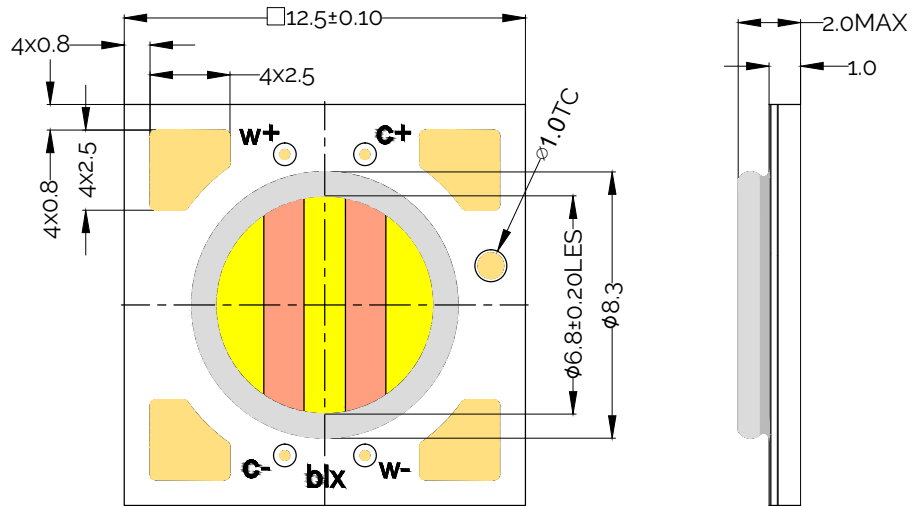
Figure 14: Drawing for Vesta Series Tunable White Gen 2 6mm Array
