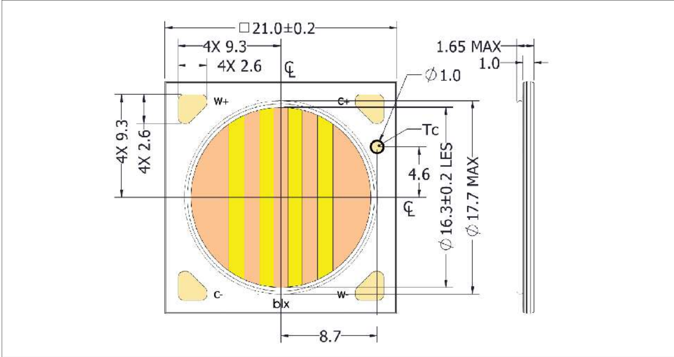
Figure 14: Drawing for Vesta Series Tunable White Gen 2 15mm Array
