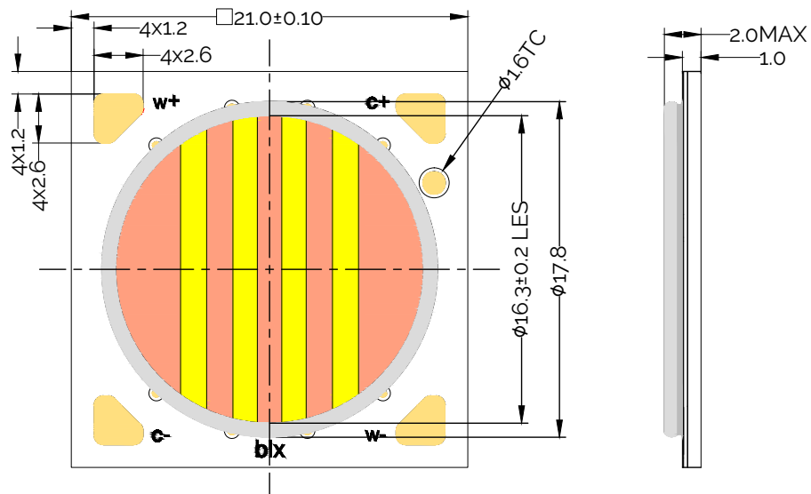
Figure 14: Drawing for Vesta Series Tunable White Gen 2 15mm Array
