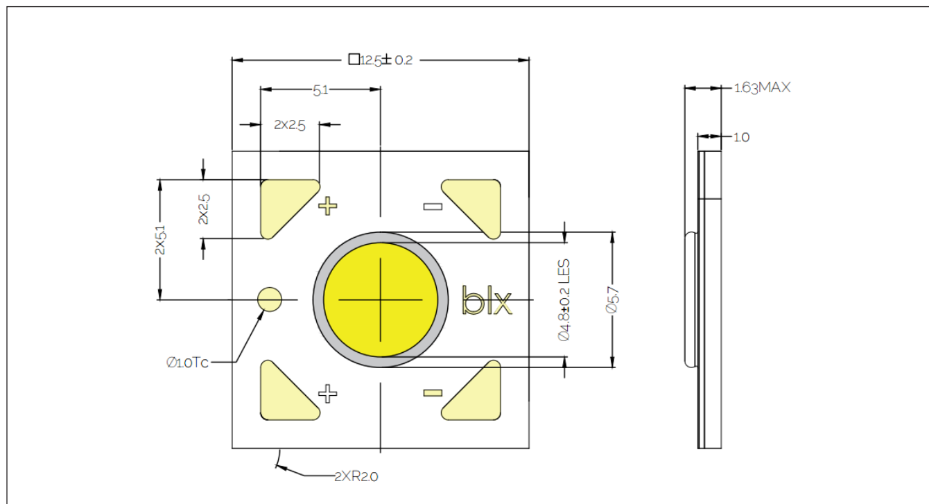
Figure 14: Drawing for V4 HD LED Array
