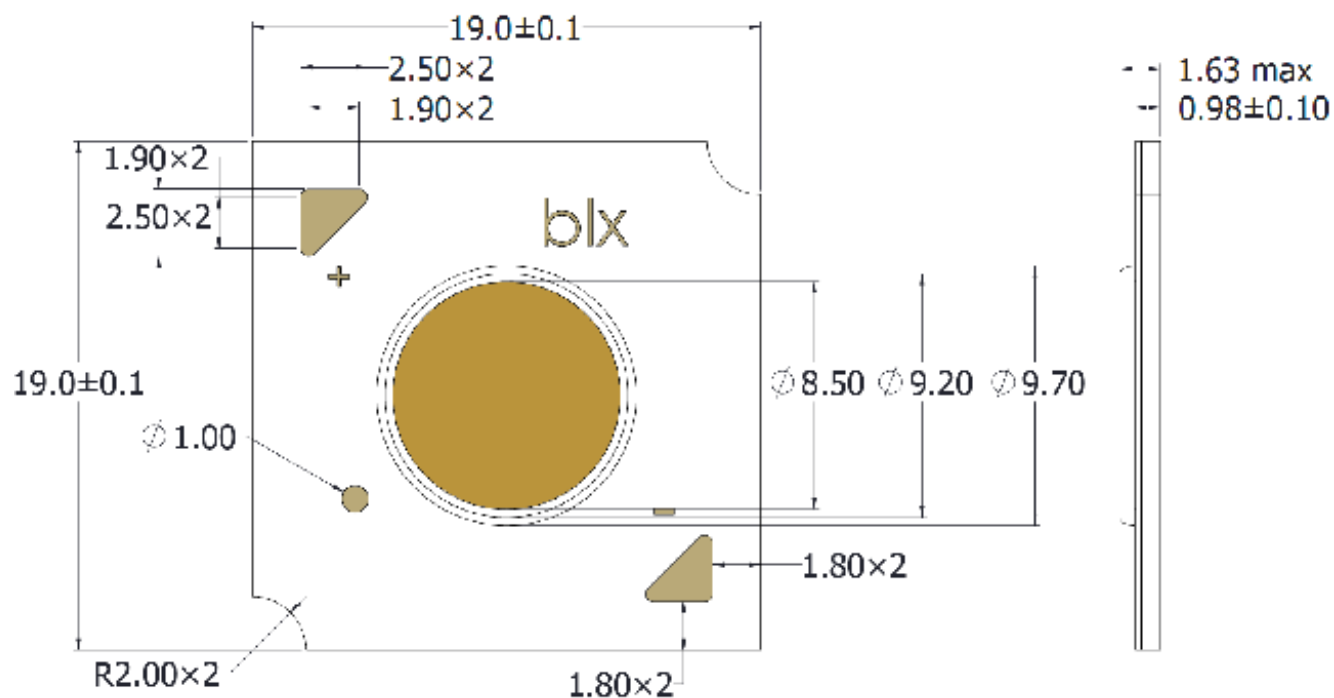
Figure 14: Drawing for Vg HD LED Array
