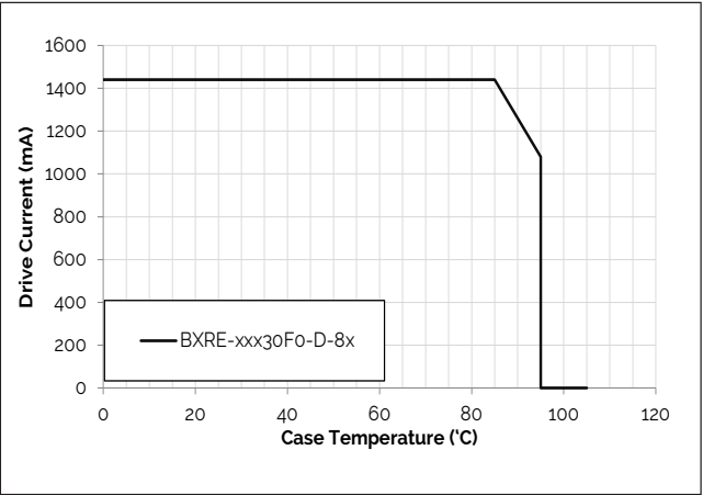
Figure 8: Derating Curve
