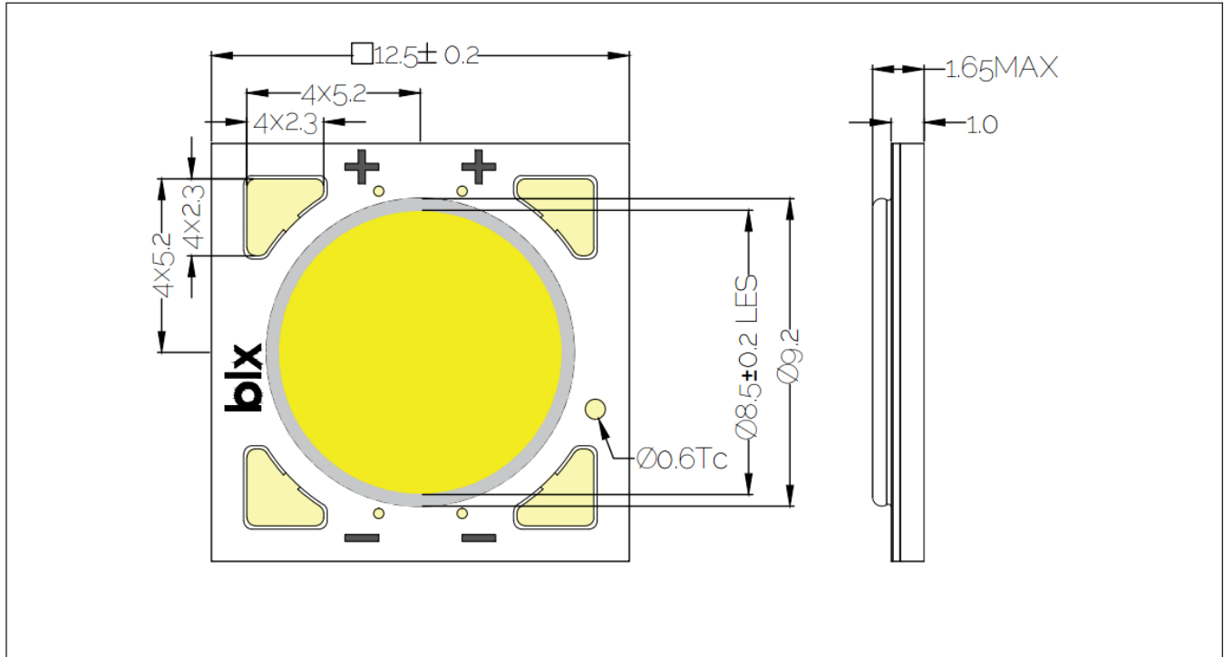
Figure 16: Drawing for V8 LED Array
