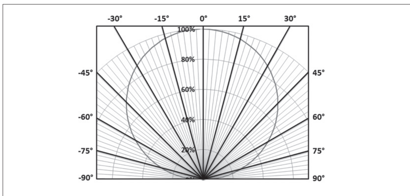
Figure 14: Typical Polar Radiation Pattern
