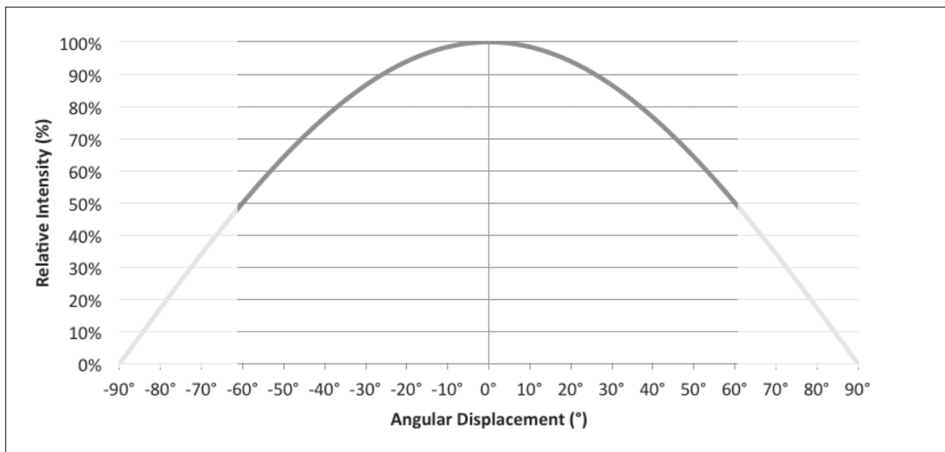
Figure 13: Typical Spatial Radiation Pattern
