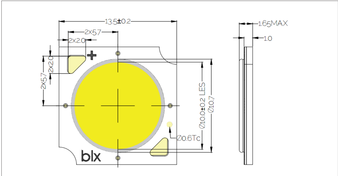
Figure 8: Drawing for V10 LED Array
