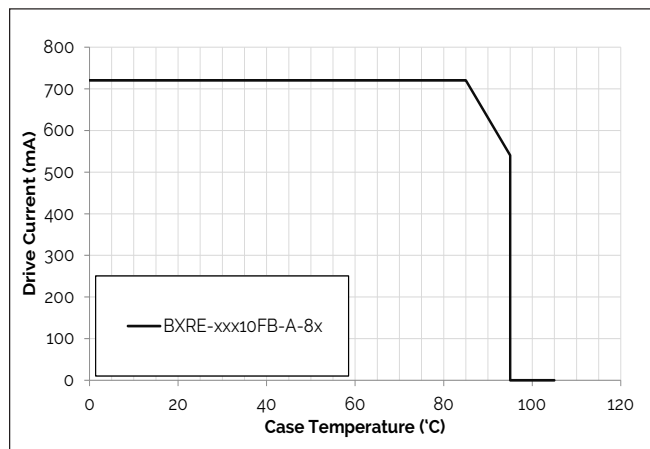
Figure 4: Derating Curve
