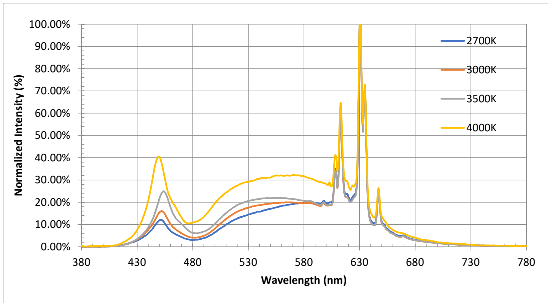
Figure 7: Typical Color Spectrum
