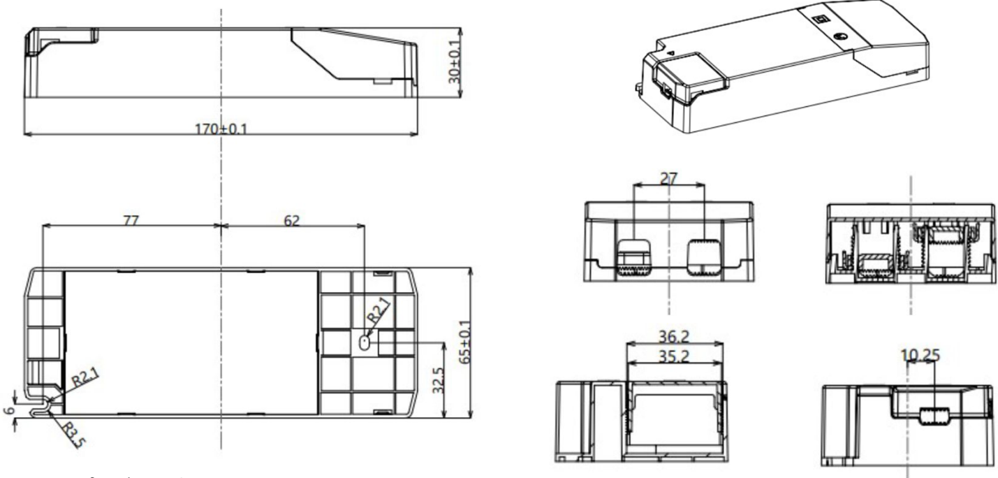
Figure 6: Mechanical Drawing
