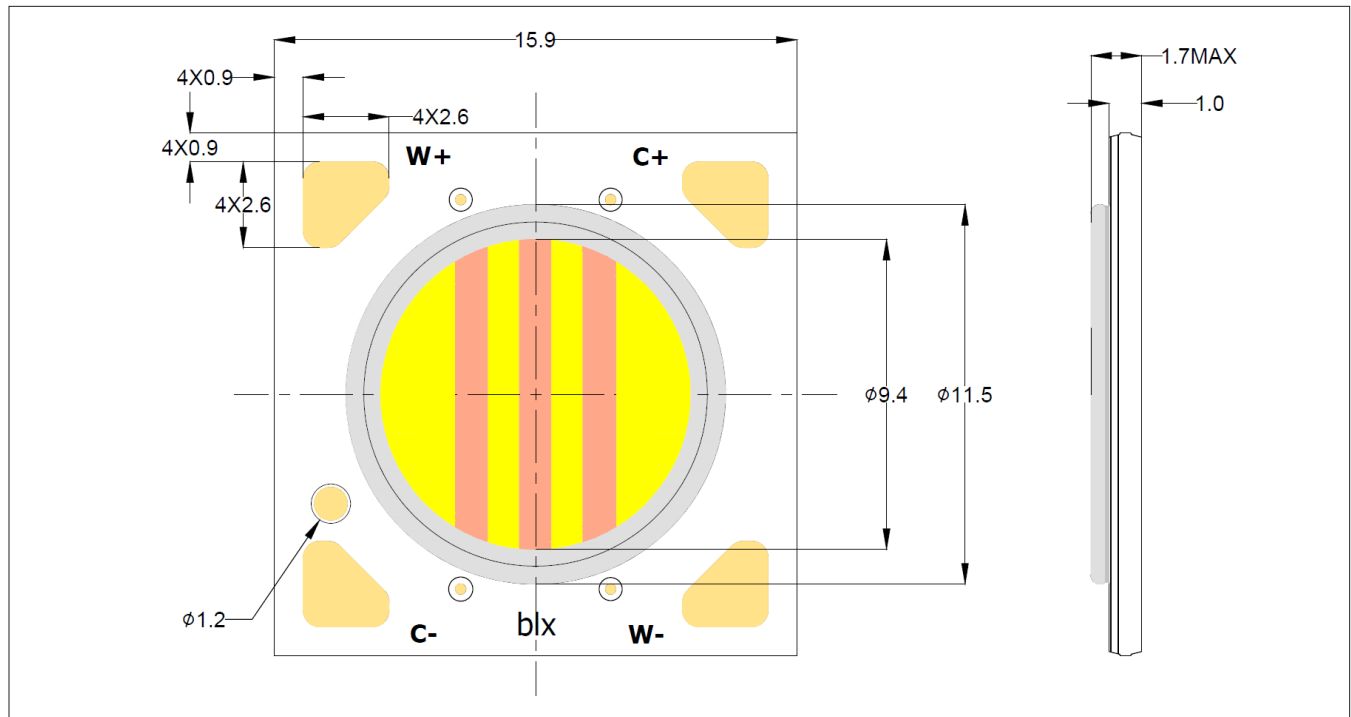
Figure 11: Drawing for Vesta Series Tunable White gmm Array
