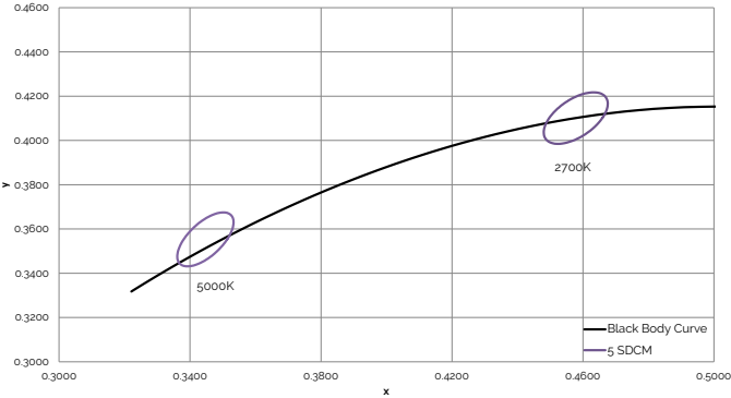
Figure 12: Graph of Test Bins in xy Color Space
