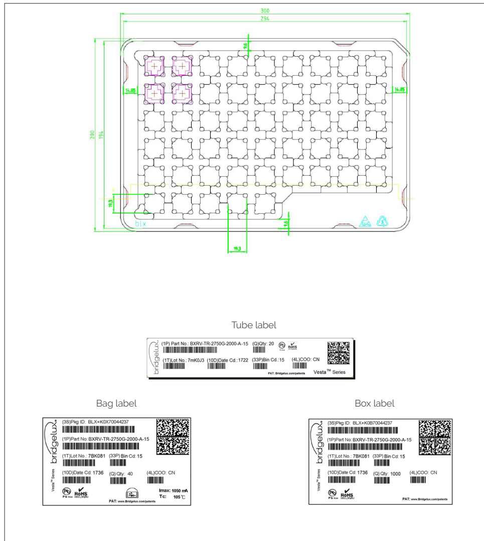
Figure 13: Vesta Series Tunable White 13mm Packaging and Labeling
