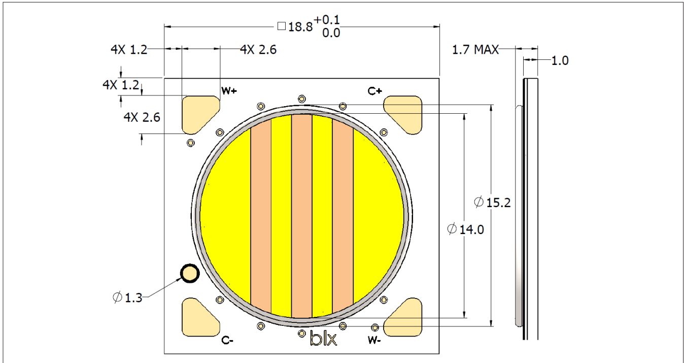
Figure 11: Drawing for Vesta Series Tunable White 13mm Array
