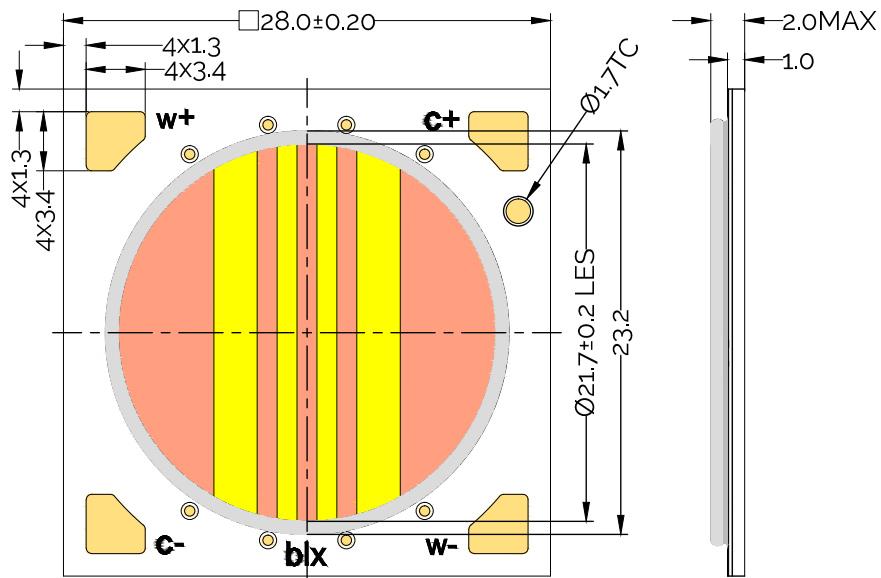
Figure 14: Drawing Specifications
