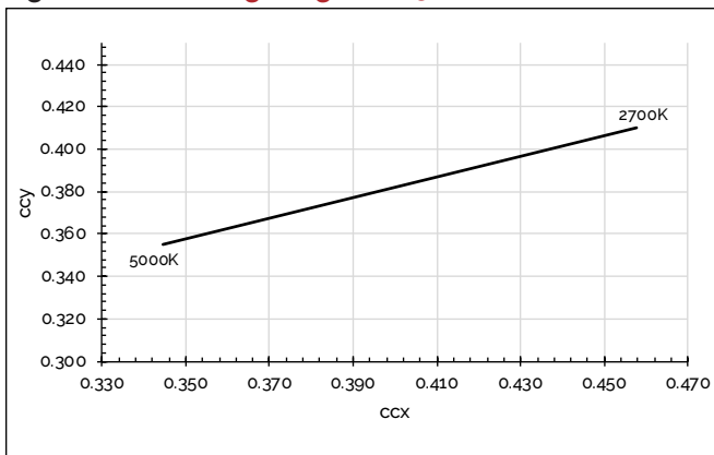
Figure 8: CCT Tuning Range, Tc=85
