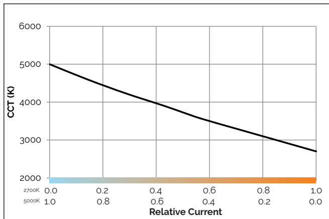
Figure 5: CCT vs. Relative Current
