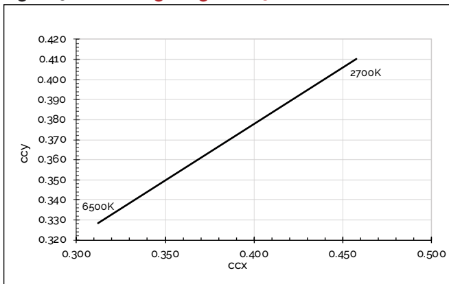
Figure 9: CCT Tuning Range, Tc=85
