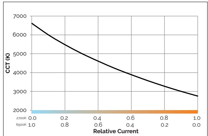
Figure 6: CCT vs. Relative Current
