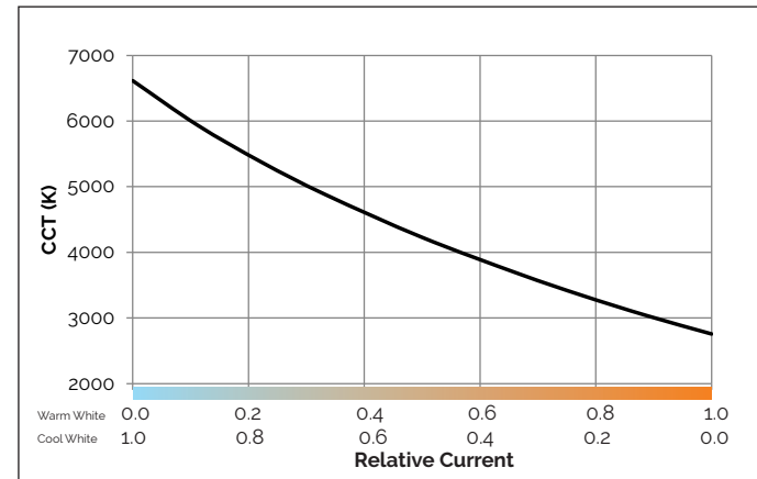
Figure 6: CCT vs. Relative Current
