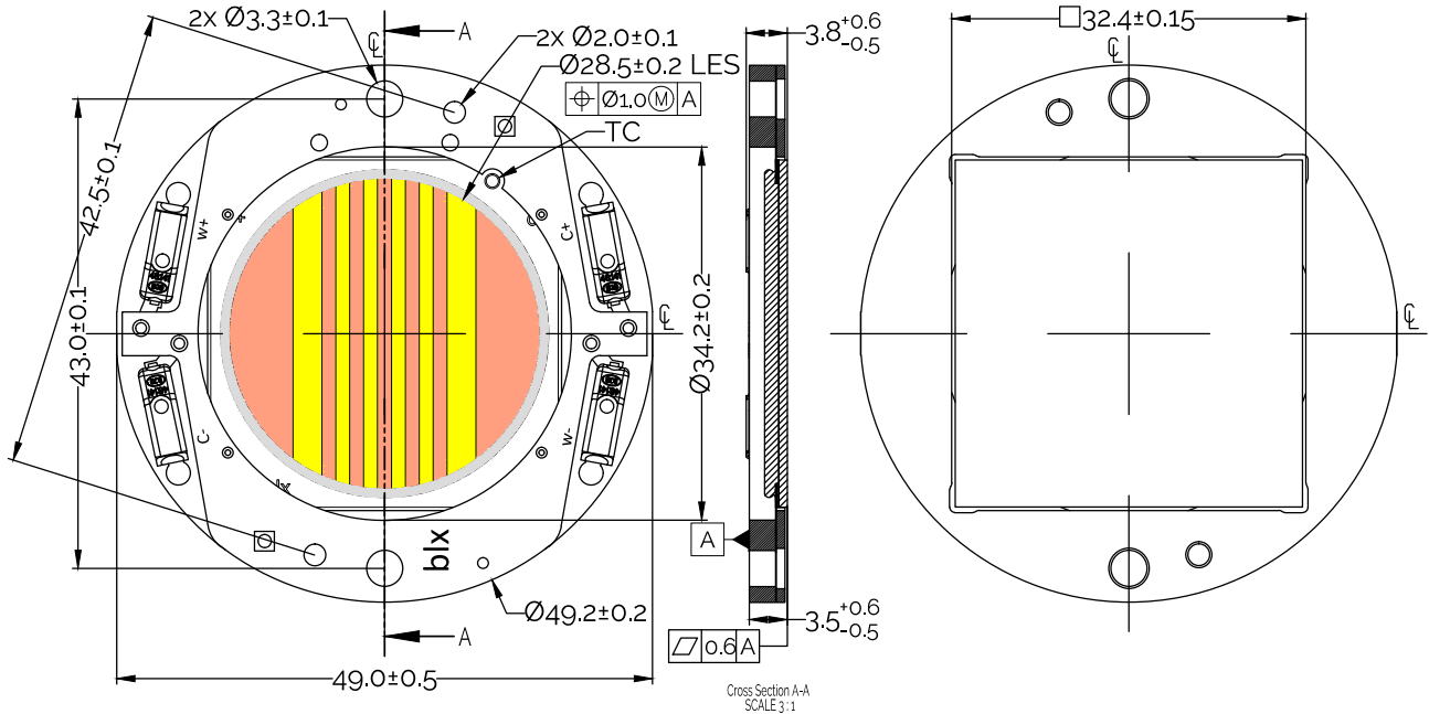
Figure 14: Mechanical Drawing Specifications
