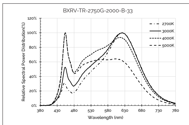
Figure 17: 2700K - 5000K with 90 CRI
