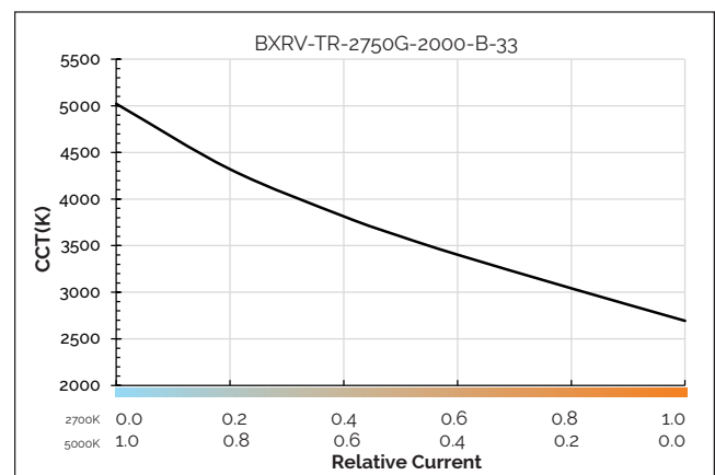
Figure 6: CCT vs. Relative Current
