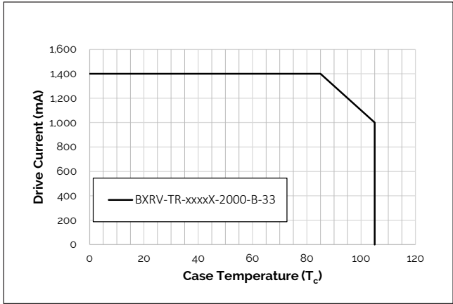
Figure 13: Derating Curve
