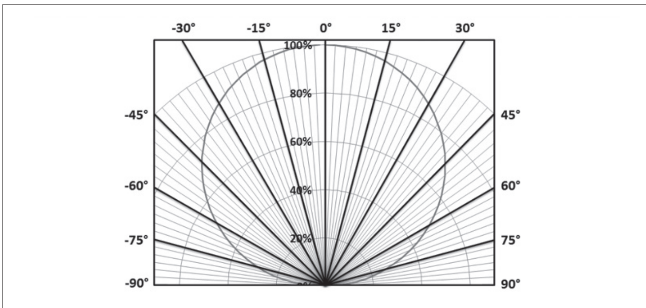
Figure 33: Typical Polar Radiation Pattern
