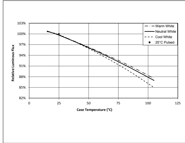
Figure 26: Vero 13 Typical DC Flux vs. Case Temperature 1
